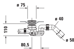
Siphon with base inlet for whirltub # 760431
