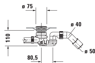
Siphon with base inlet for bathtub # 700432
