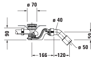
Siphon for bathtub # 700432
