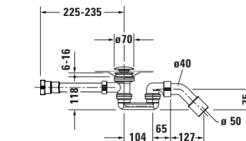
Siphon for bathtub # 700434
