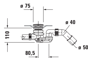
Siphon with base inlet for whirltub # 760432
