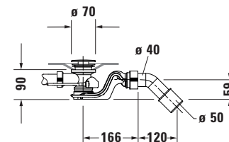
Siphon for bathtub # 700433
