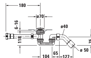
Siphon for bathtub # 700434
