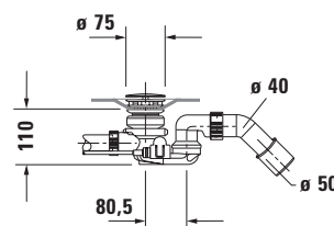
Siphon with base inlet for bathtub # 700433
