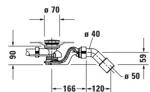
Siphon for whirltub # 760431
