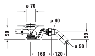
Siphon for whirltub # 760432
