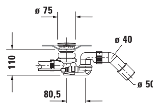
Siphon with base inlet for whirltub # 760433
