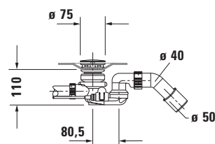
Siphon with base inlet for bathtub # 700431
