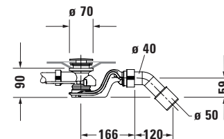
Siphon for bathtub # 700431
